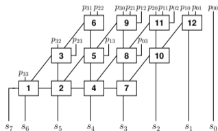
Column-wise Order
