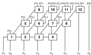
Row-wise Order
